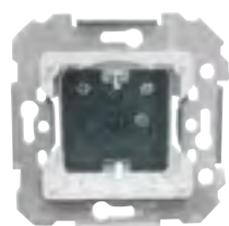
Schuko® 2P+E socket outlet (lateral earthing) with safety protection Screwed terminals 16 A 250 V~
