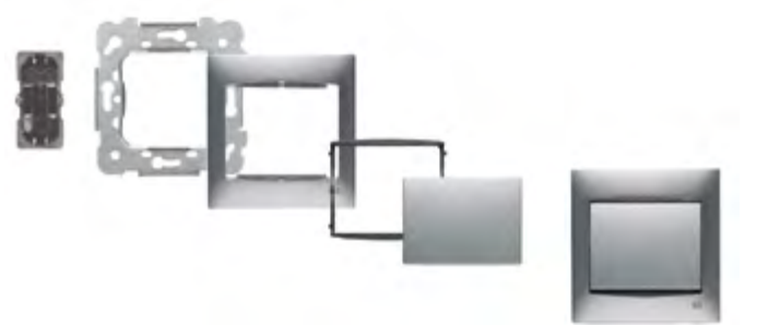
16505 + 16-BAST + 21011-PL + 21600-NIM + 21705-PL Single pole one-way switch
